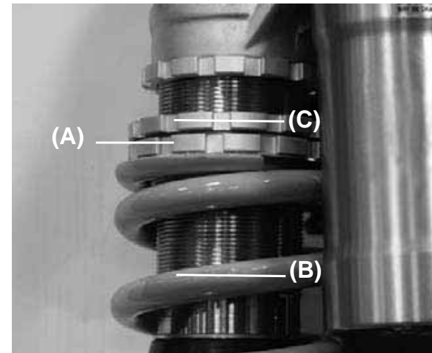
(A). Nut. (B). Spring. (C). Locknut.
